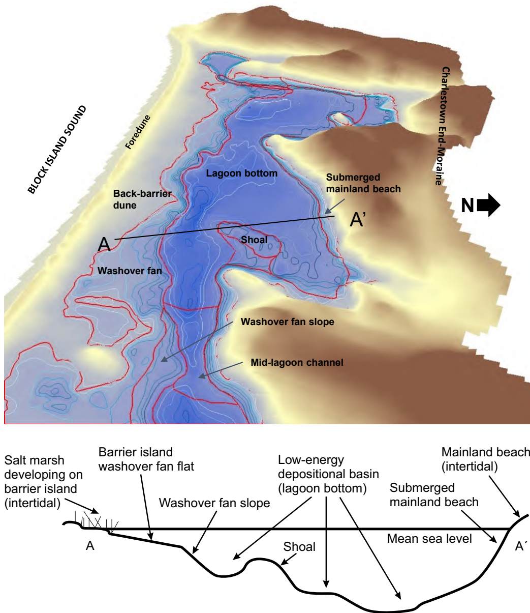
Examples of subaqueous landscape units across a coastal lagoon.
