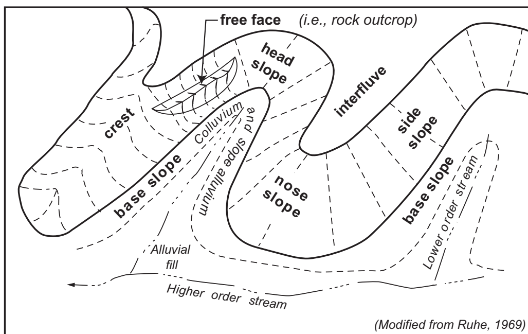
Three-dimensional depiction of geomorphic components of hills.
